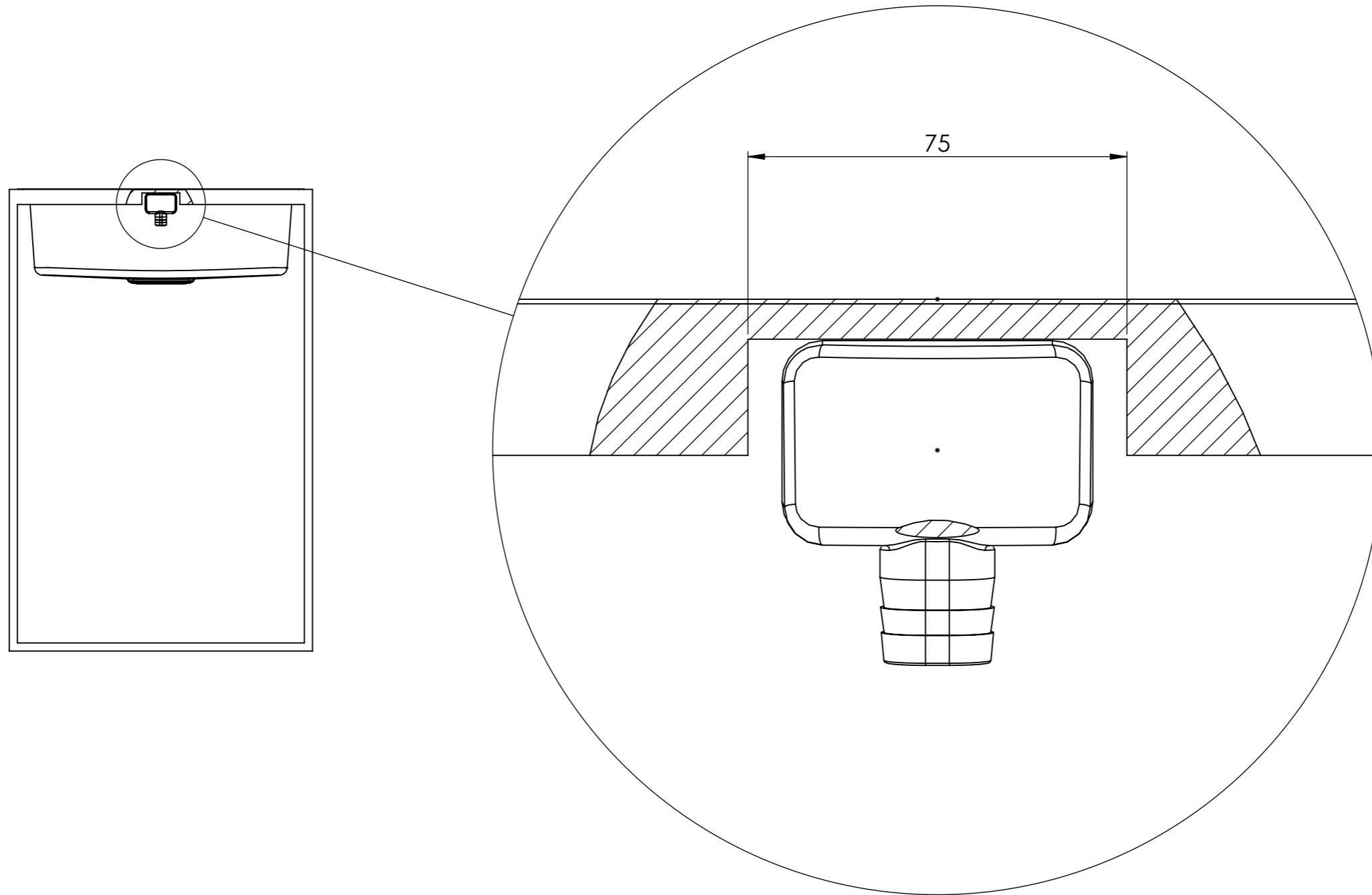
DETAIL AD SCALE 1 : 1
